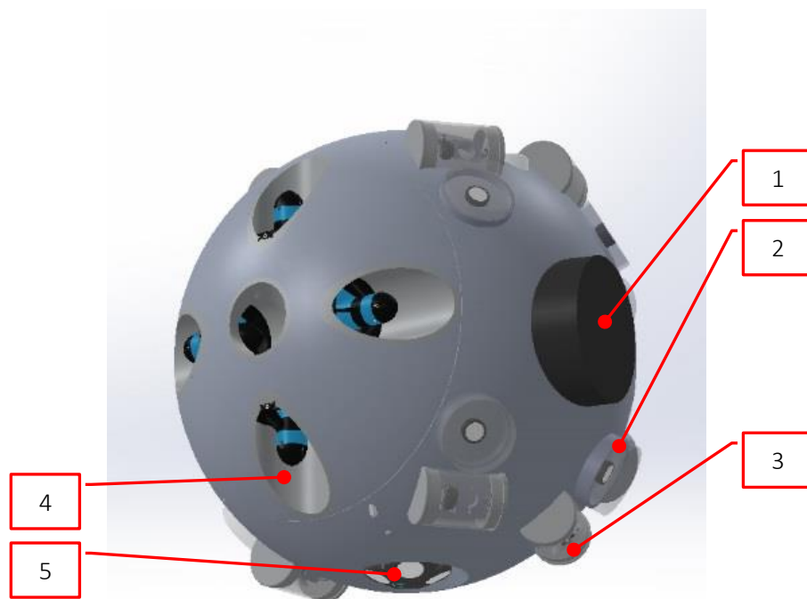
Figure 1-1 3D CAD model of UX-1
